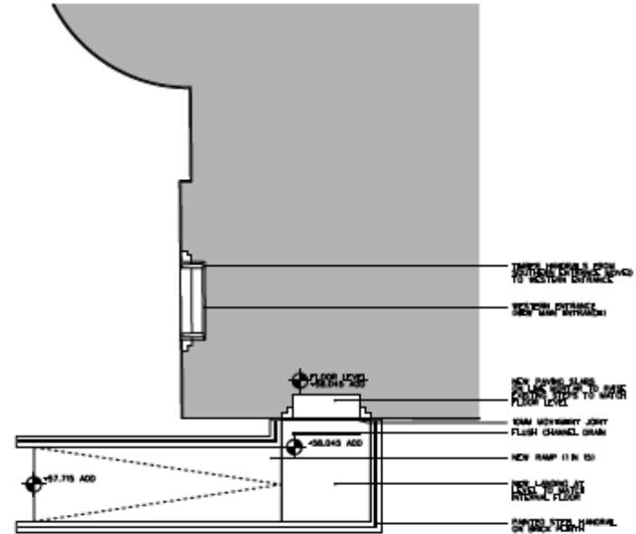
02 PROPOSED PLAN SCALE 1/50
