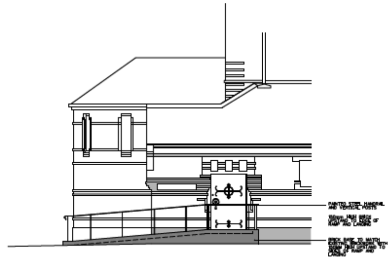
04 PROPOSED ELEVATION SCALE 1/50
